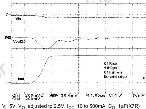
Figure 23 : Load Transient
